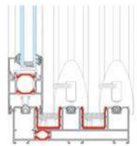
Triple Track
