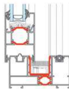
Double Track
