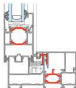
Single Track
