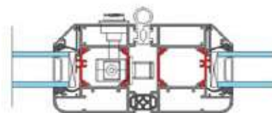
Interlock Detail
